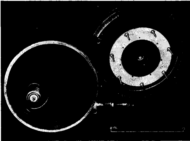
FIG. 8-6.—Photograph of a parallel-pin rotary gap.
